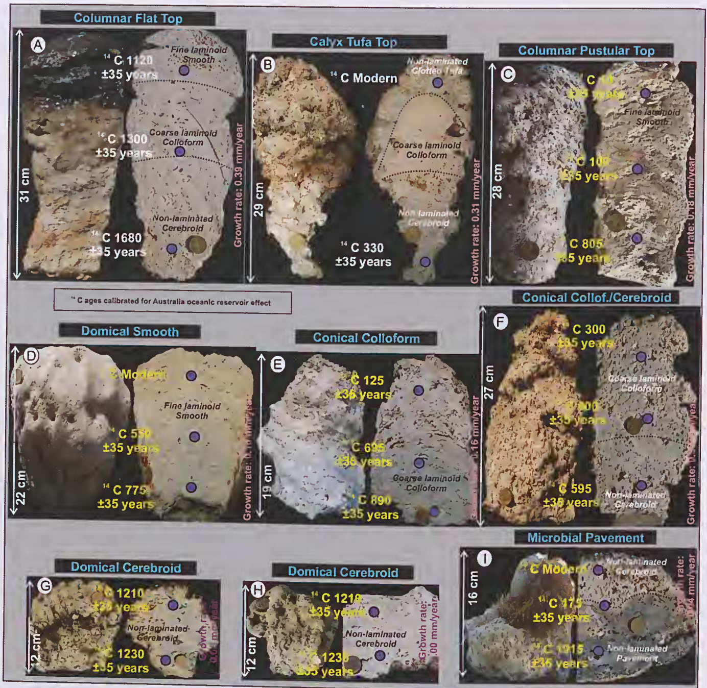
Figure 17 Microbial buildup slices showing internal fabrics, the sampling points and calibrated ^{14}\text{C} ages with growth rates. (A) Columnar flat top structure with an internal shallowing-upward carbonate sequence represented by a basal non-laminated fabric passing upward to coarse laminoid and to fine laminoid fabric. (B) Calyx head with ornamented non-laminated fabric at top. (C) Columnar head with internal fine laminoid fabric and colonised by pustular at surface. (D) Domical structure with smooth top and internal fine laminoid fabric. (E) Conical colloform structure with a coarse laminoid internal fabric. (F) Conical structure with non-laminated fabric at base passing upward to a coarse laminoid fabric, (G, H) Domical cerebroid structure with internal non-laminated fabric. (I) Microbial pavement with a non-laminated fabric passing upward to a cerebroid morphology. (Jahnert & Collins 2012 figure 12).
